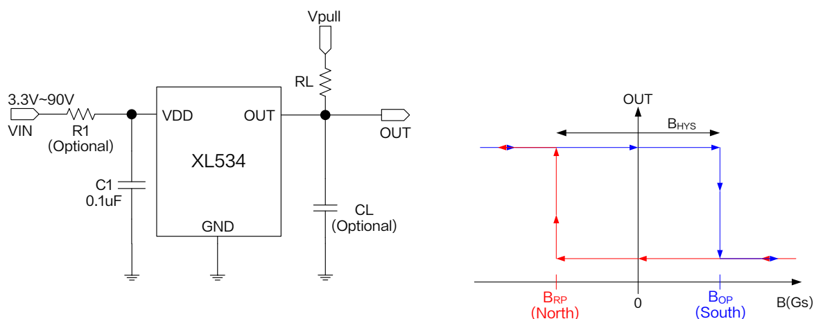
Figure1.XL534 Typical application schematic and output characteristic curve
