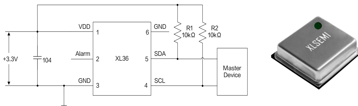
Figure1. XL36 Typical application schematic and Package Type
