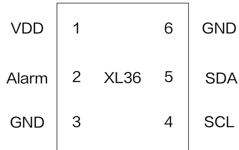
Figure2. Pin Configuration of XL36
