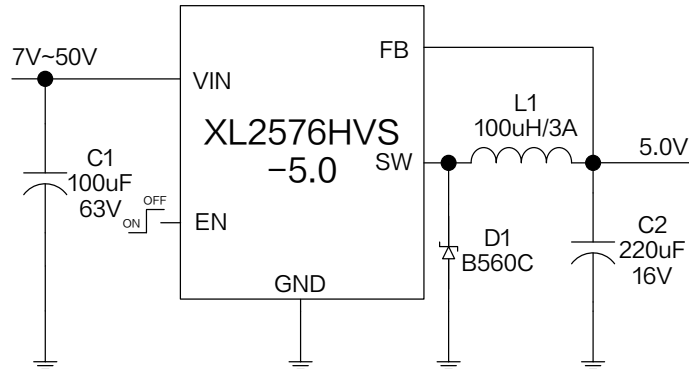
Figure8. XL2576HVS-5.0 System Parameters Test Circuit
