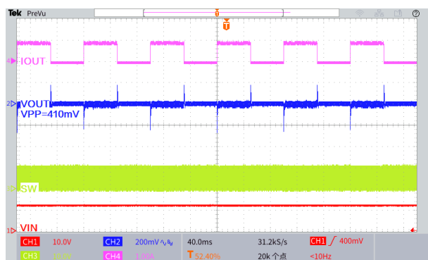
Figure30. Load Transient Response ( V_{IN}=12V , V_{OUT}=5.0V , I_{OUT}=0.1 to 1A )
