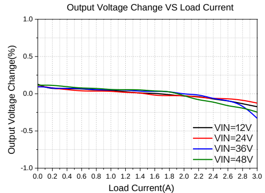
Figure13.Load Regulation
