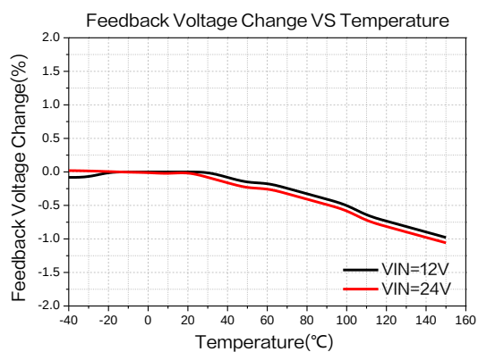
Figure16.Feedback Voltage Regulation
