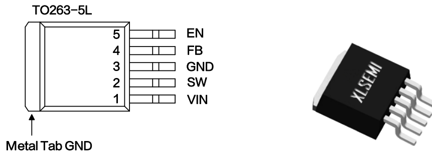
Figure2. Pin Configuration of XL2576HVS
