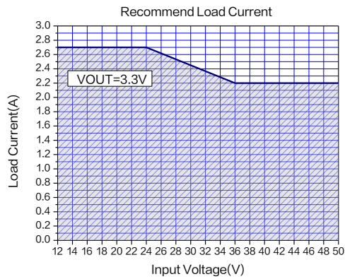
Figure18.Max Output Current ( V_{OUT}=3.3V , T_A=25^{\circ}C )
