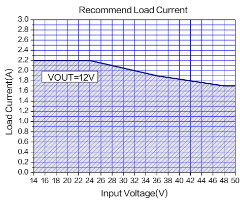
Figure20.Max Output Current ( V_{OUT}=12V , T_A=25^{\circ}C )
