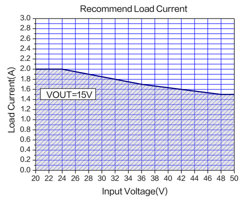
Figure21.Max Output Current ( V_{OUT}=15V , T_A=25^{\circ}C )
