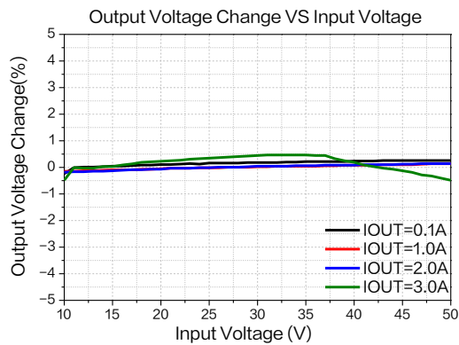
Figure12.Line Regulation
