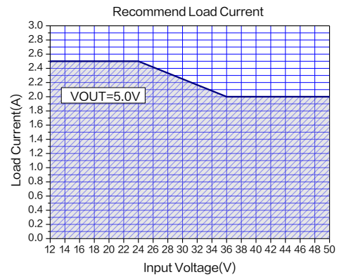
Figure19.Max Output Current ( V_{OUT}=5.0V , T_A=25^{\circ}C )
