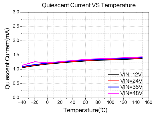
Figure17. Quiescent Current
